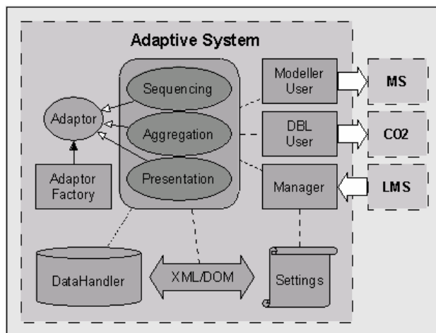
Figure 3: Implementation details of the Adaptive System
