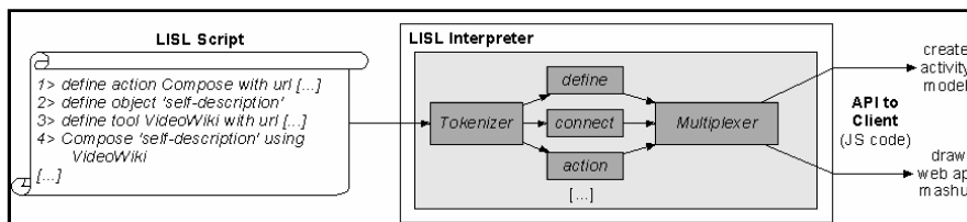
Fig. 3. Functional diagram of the LISL interpreter including a tokenizer, interpreter units for each statement type, and a multiplexer controlling different APIs
