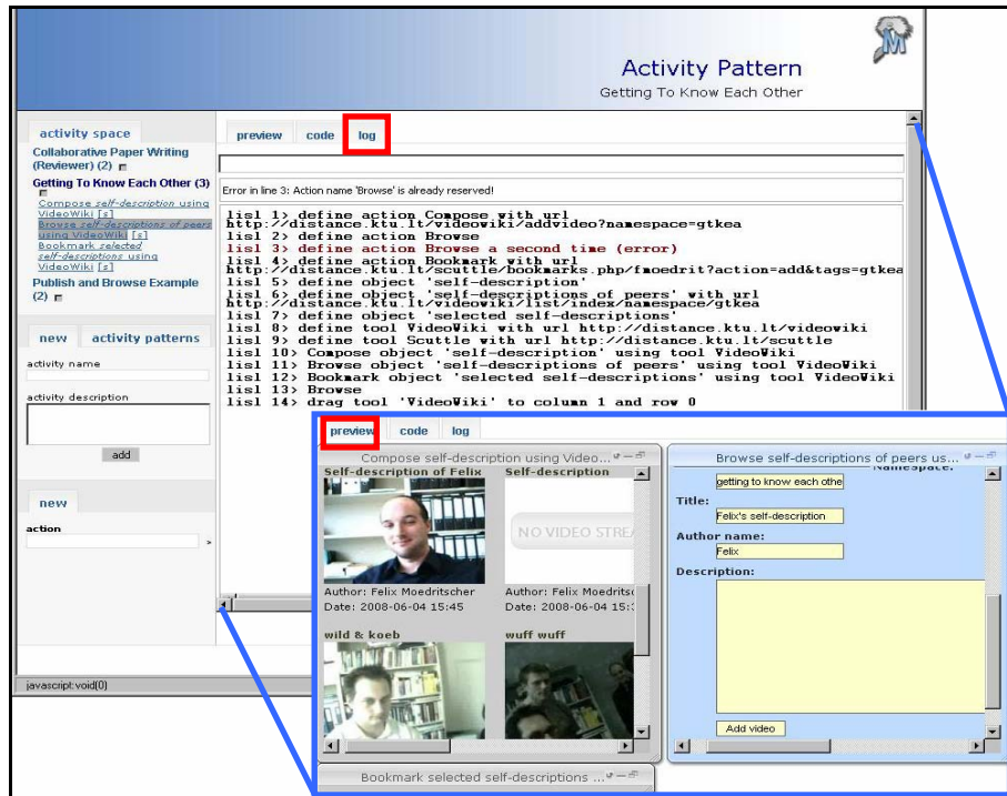
Fig. 4. MUPPLE page for the activity ‘Getting To Know Each Other’; the tab ‘log’ shows the LISL script of our example executed by the interpreter (red indicates an error), while the tab ‘preview’ (blue border) visualizes the web application mashup and provides web-based widgets
